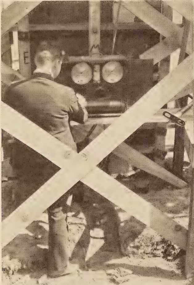
FIGURE 3.—AUXILIARY EQUIPMENT USED WITH PRESSURE CELLS
